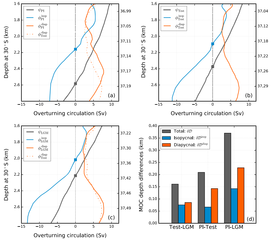
Figure 2. (a–c) Meridional Overturning Circulation (MOC) streamfunction components \psi(30^\circ\text{S}, \sigma_2) , \phi^{\text{isop}}(\sigma_2) , and \phi^{\text{diap}}(\sigma_2) , mapped to depth coordinates using the mean isopycnal depth at 30^\circ\text{S} (see details in section 4), with corresponding potential densities \sigma_2 labeled on the right axis, for each simulation. The three solid curves in each panel can be interpreted as follows: the black line shows the simulated overturning circulation streamfunction at 30^\circ\text{S} , the blue line ( \phi^{\text{isop}} ) shows the MOC streamfunction that would occur at 30^\circ\text{S} if the circulation were purely adiabatic below z_{\text{ref}} in the Southern Ocean, and the red line ( \phi^{\text{diap}} ) shows the difference between \psi and \phi^{\text{isop}} . Hence, \phi^{\text{diap}} quantifies the along-isopycnal change in the MOC streamfunction due to diapycnal mixing below z_{\text{ref}} = -1.5 km in the Southern Ocean. The \phi^{\text{diap}} curve in the Test run is repeated for comparison in panels (a) and (c) as a dash-dotted red line. The MOC depths corresponding to \psi(30^\circ\text{S}, \sigma_2) and \phi^{\text{isop}} are indicated in each panel by the blue and black squares, respectively. (d) Contribution to the inter-simulation differences in the MOC depths (black) due to changes in shapes of isopycnals and surface forcing (blue) and due to changes in deviations of the MOC depth from isopycnals (red). See section 4 for definitions of \delta D , \delta D^{\text{isop}} , and \delta D^{\text{diap}} . In order to avoid the influence of grid-level noise, the smoothed MOC streamfunction shown in Figure 1 is used here. An equivalent figure that instead uses the raw unsmoothed MOC streamfunction is included in the supporting information (Figure S10). PI = preindustrial; LGM = Last Glacial Maximum.
